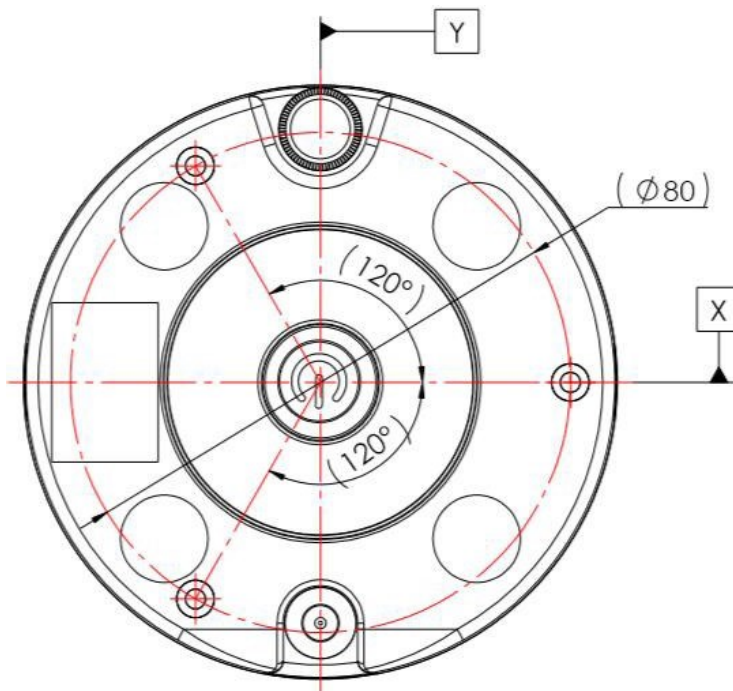
Position of M4 screw threads:
